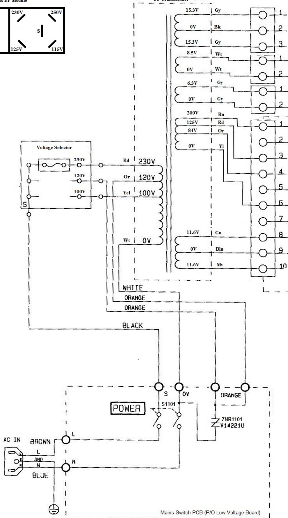
I/P Transformer
